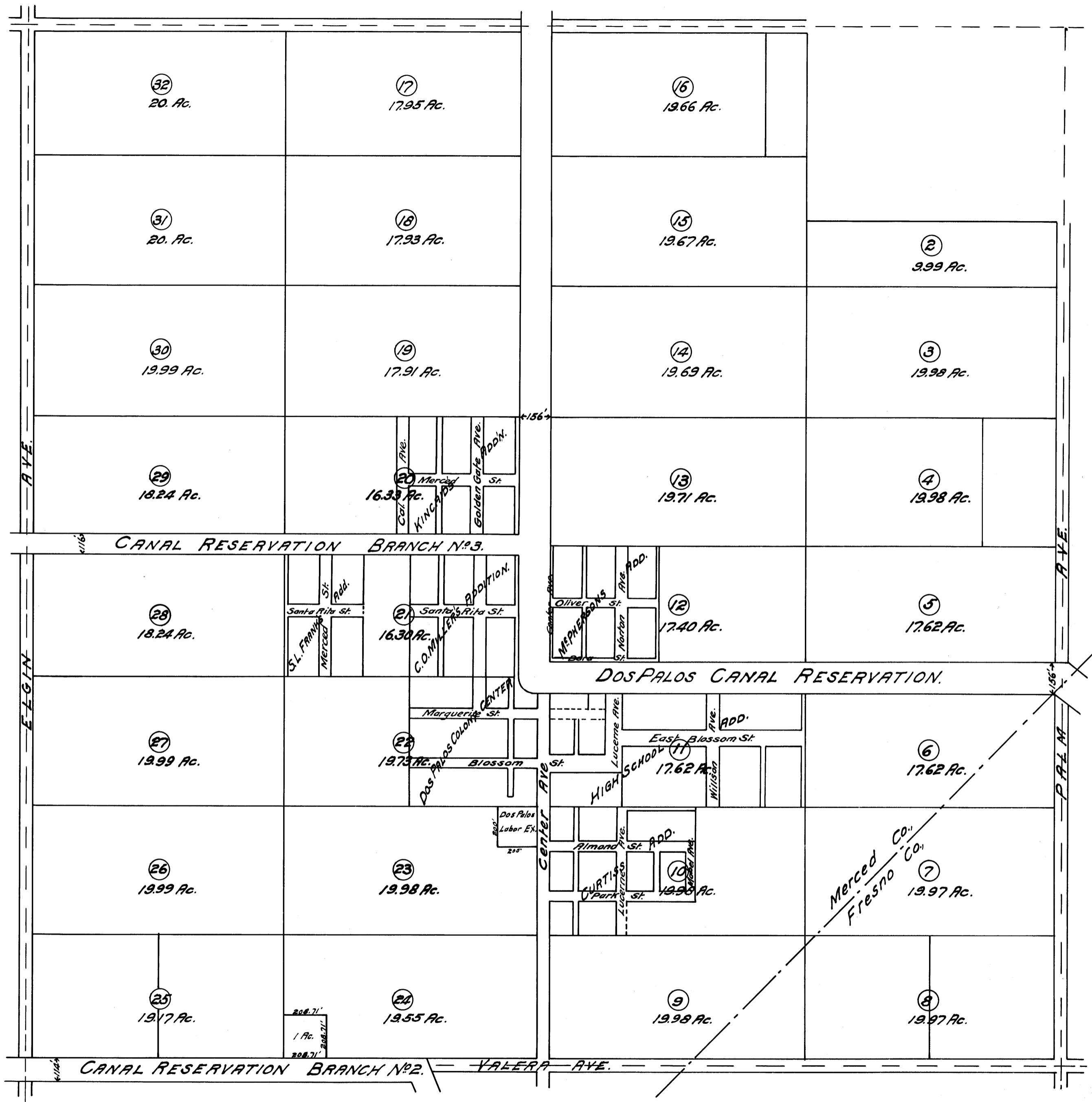
MAP OF MILLER AND LUX SUBDIVISION OF SECTION 11, T.11S. R.12E., M.D.M., Surveyed by H. Wanzer, 1895. Platted by C. B. Gleaves, Jan. 28, 1909.
