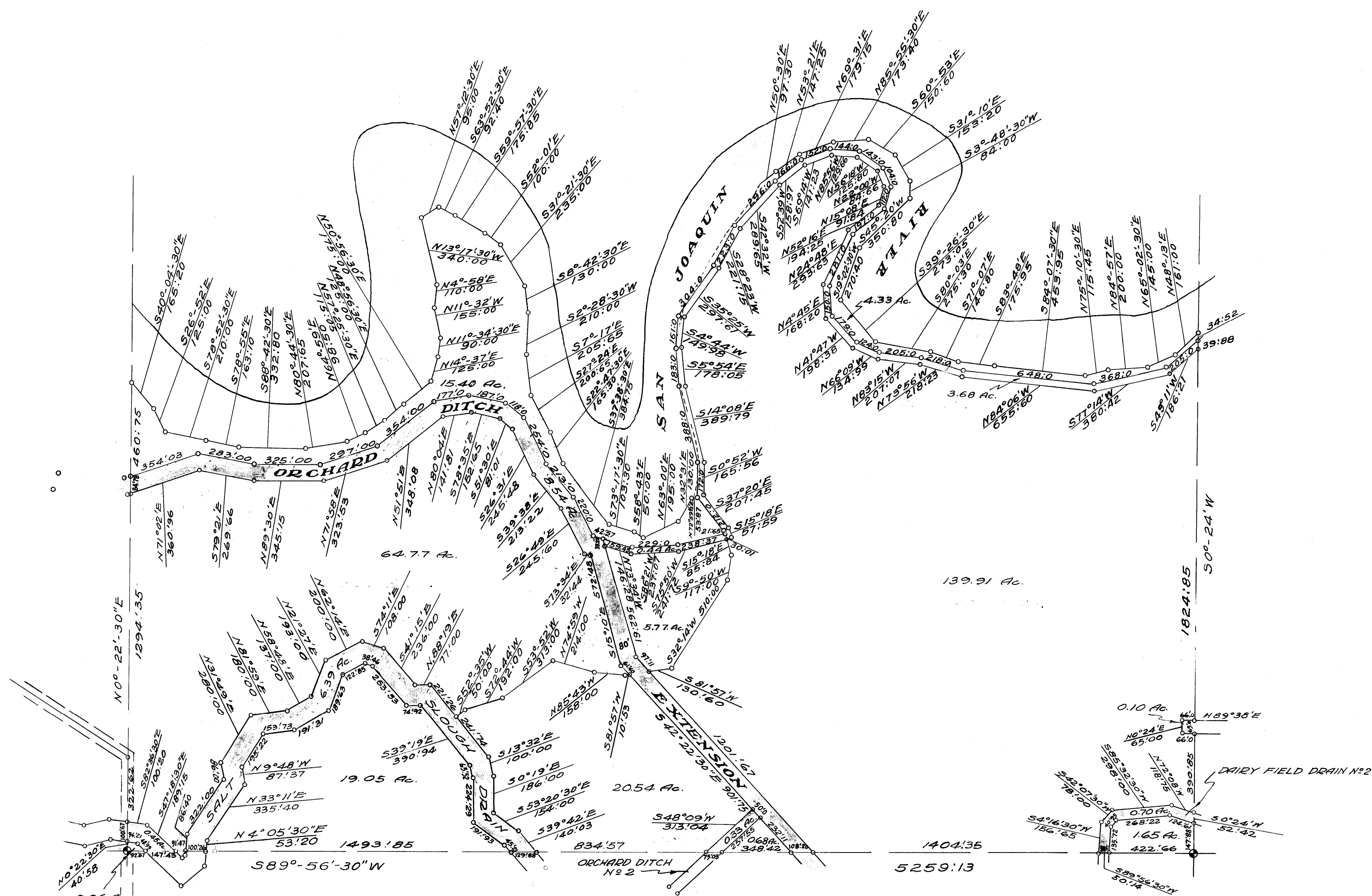
MILLER & LUX SUBDIVISION SECT. 26 T 9 S, R 12 E MERCED COUNTY SCALE 1 IN. = 400 FT.
